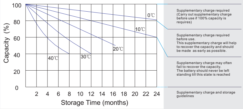
Storage characteristic
